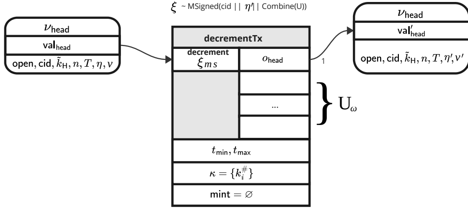
Figure 10: decrement transaction spending an open head output, producing a new head output and multiple decommitted outputs.
