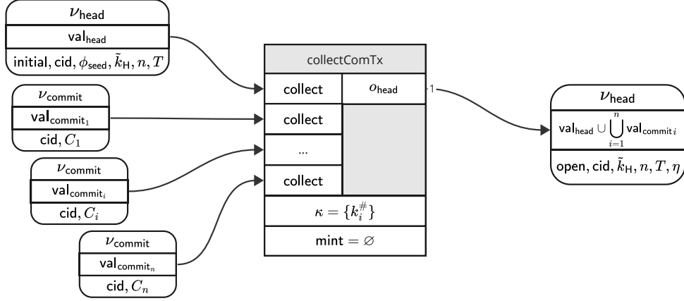
Figure 6: collectCom transaction spending the head output in initial state and collecting from multiple commit outputs into a single open head output.
