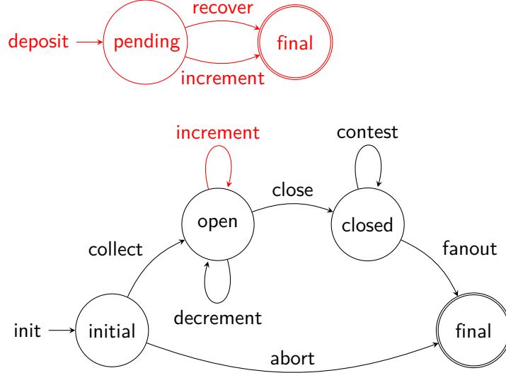
Figure 1: Mainchain state diagram for this version of the Hydra protocol.
