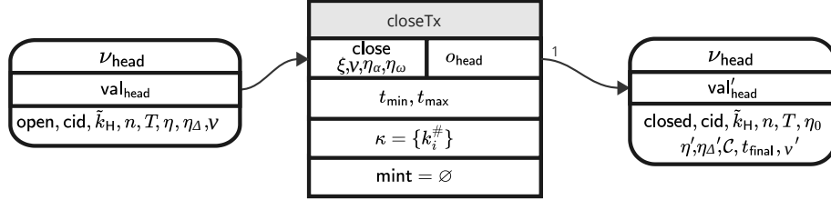
Figure 11: close transaction spending the open head output and producing a closed head output.
