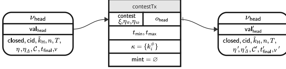
Figure 12: contest transaction spending the closed head output and producing a different closed head output.
