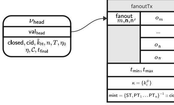
Figure 13: fanout transaction spending the closed head output and distributing funds with outputs o_1 \dots o_{m+n+n'} .
